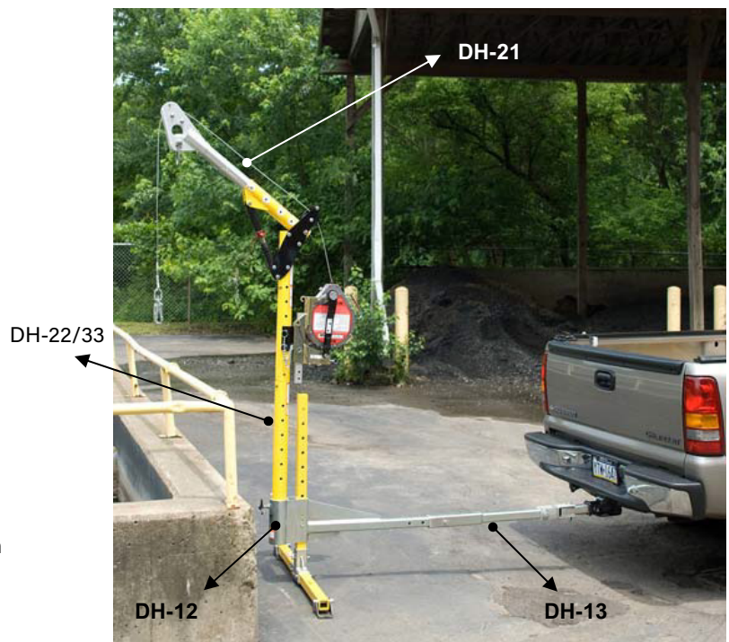
2-ft. Vehicle Hitch Mount Extension (DH-13) installed between Vehicle Hitch Mount Sleeve (DH-12) and attendant vehicle:
